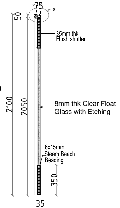
Section 2-2
